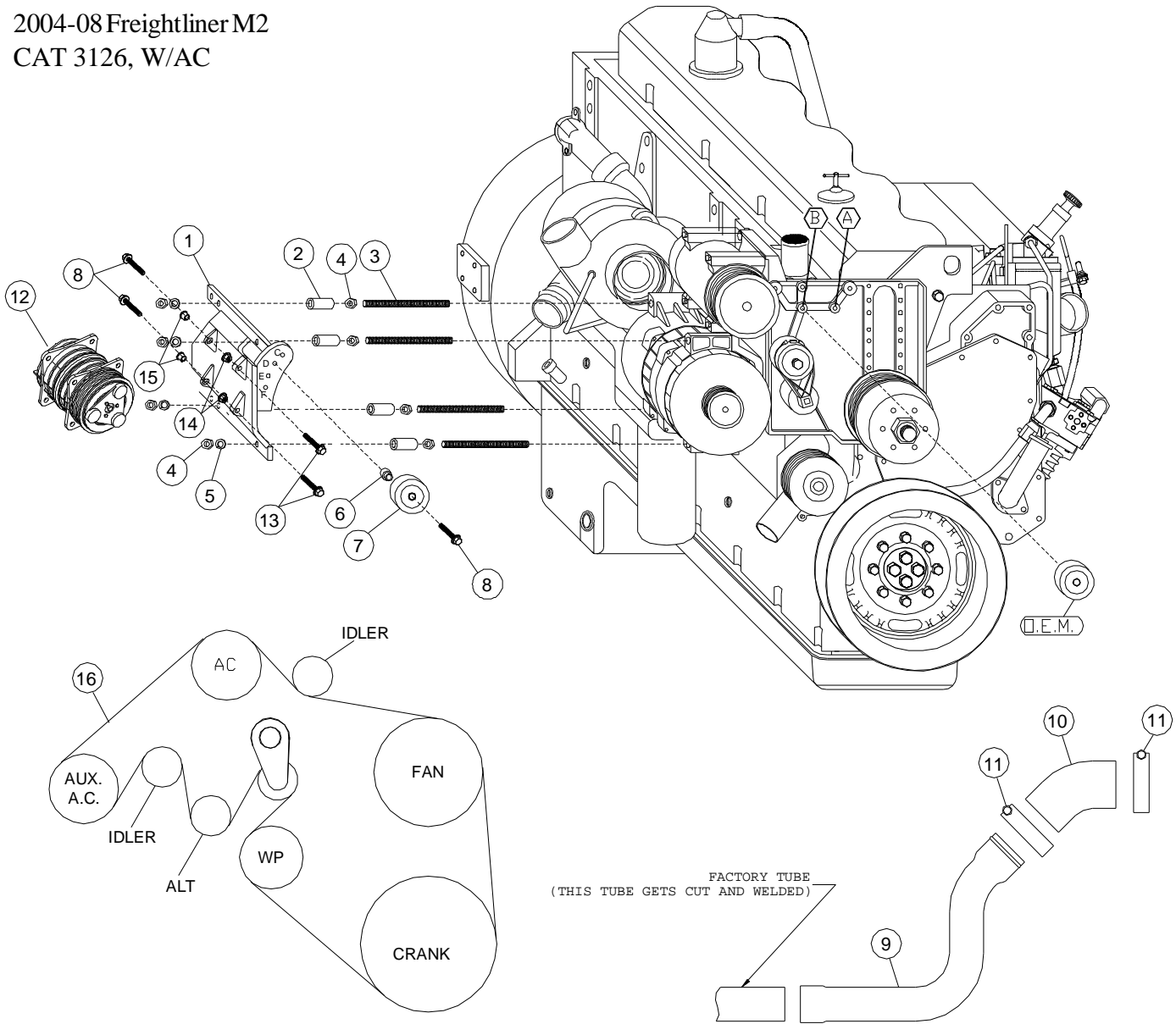
BELT DIAGRAM
