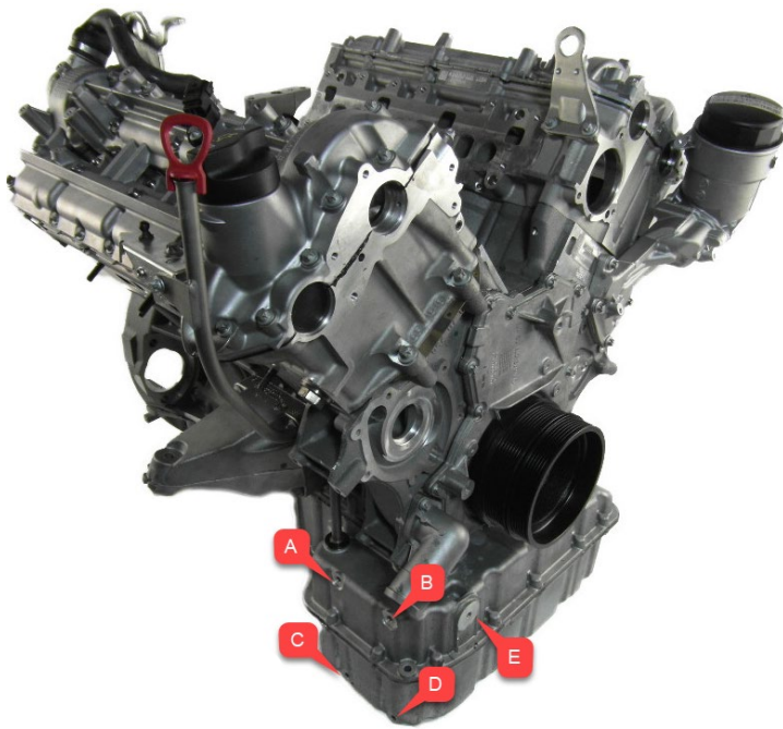
Mounting Location
