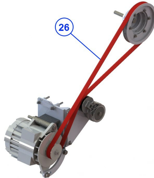
Belt Routing
