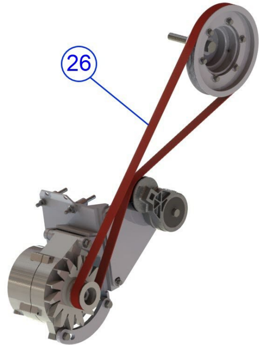
Belt Routing
