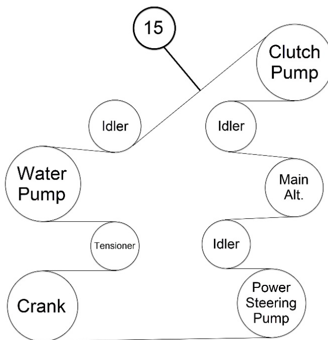
Belt Routing (15)
