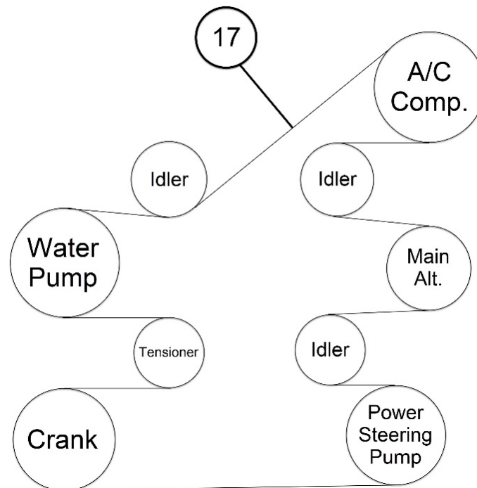
Belt Routing (17)
