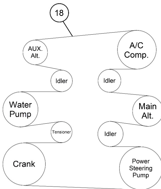
Belt Routing (18)
