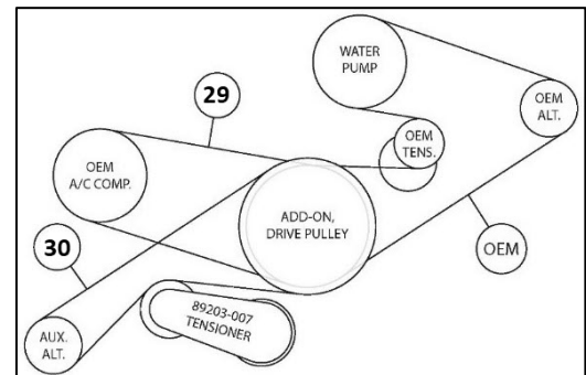
Belt Routings (29-30)
