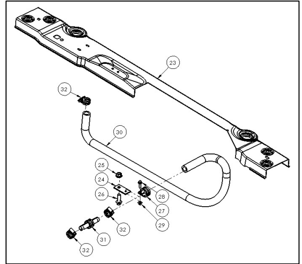
Mod. Radiator Brace (23), Heater Hose Assembly (24-32) Illustration View from Top, Back of the Engine Bay
