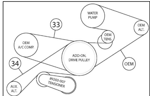
Belt Routings (33-34)
