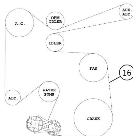
Belt Routing (16)
