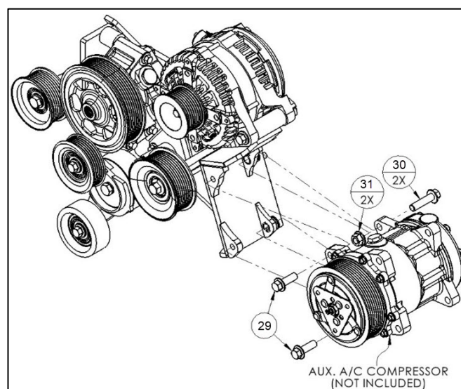
Auxiliary A/C Compressor Mounting Hardware (29-31)
