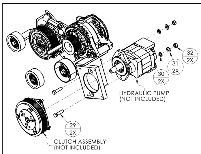
Clutch Pump Mounting Hardware (29-32)
