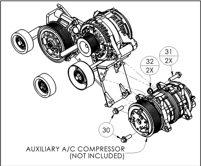
Auxiliary A/C Compressor Mounting Hardware (30-32)
