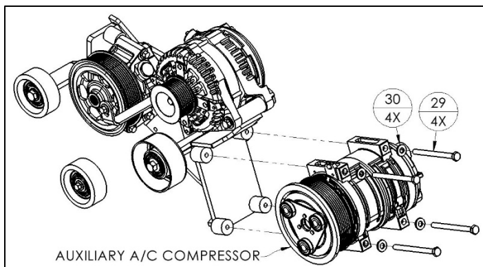
Auxiliary A/C Compressor Mounting Hardware (29-30)
