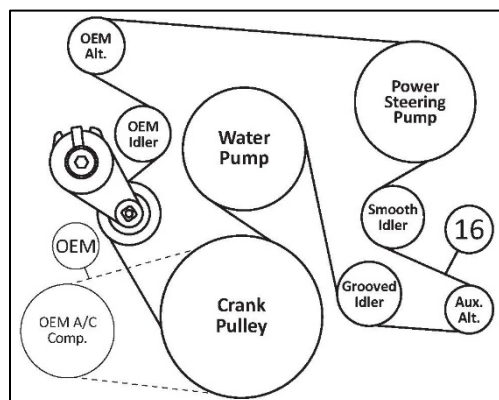
Belt Routing (16)
