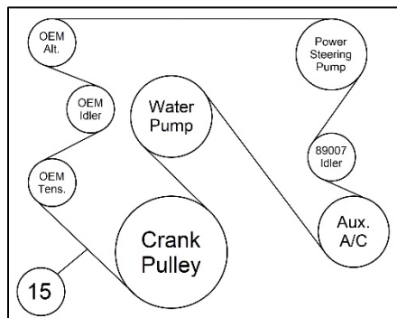
Belt Routing (15)
