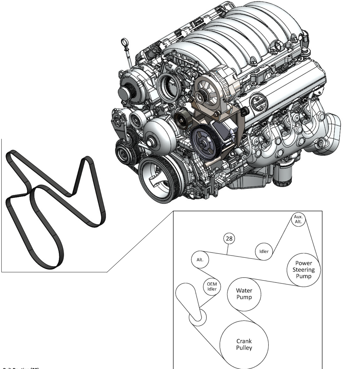
Belt Routing (28)
