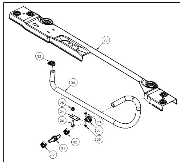
Mod. Radiator Brace (23), Heater Hose Assembly (24-32) Illustration View from Top, Back of the Engine Bay
