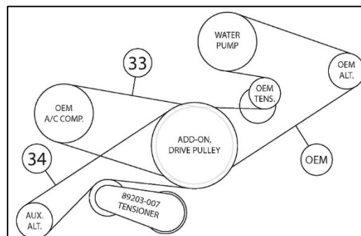
Belt Routings (33-34)
