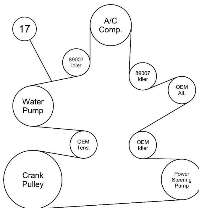
Belt Routing
